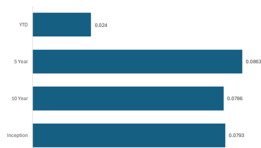
Period IRRs
